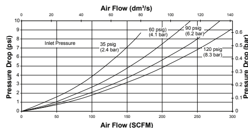
3/4" 3000 SERIES FILTER
